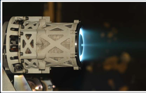
Halo12 Hall Thruster
